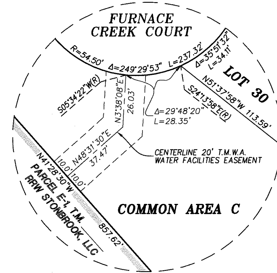
DETAIL E SCALE 1"=30'
