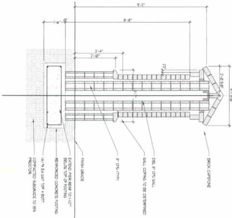
2 SECT THRU PILASTER AL-02 SCALE 1/2" = 1'-0"
