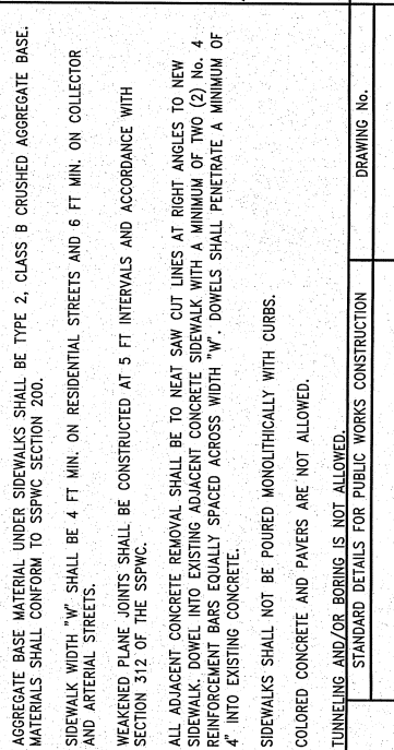
STANDARD DETAILS FOR PUBLIC WORKS CONSTRUCTION DRAWING NO. R-122 DATE: 3/2014
